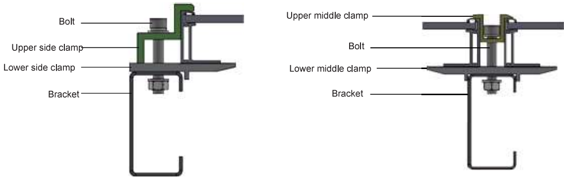
Bifacial double-glass PV module (frame)
