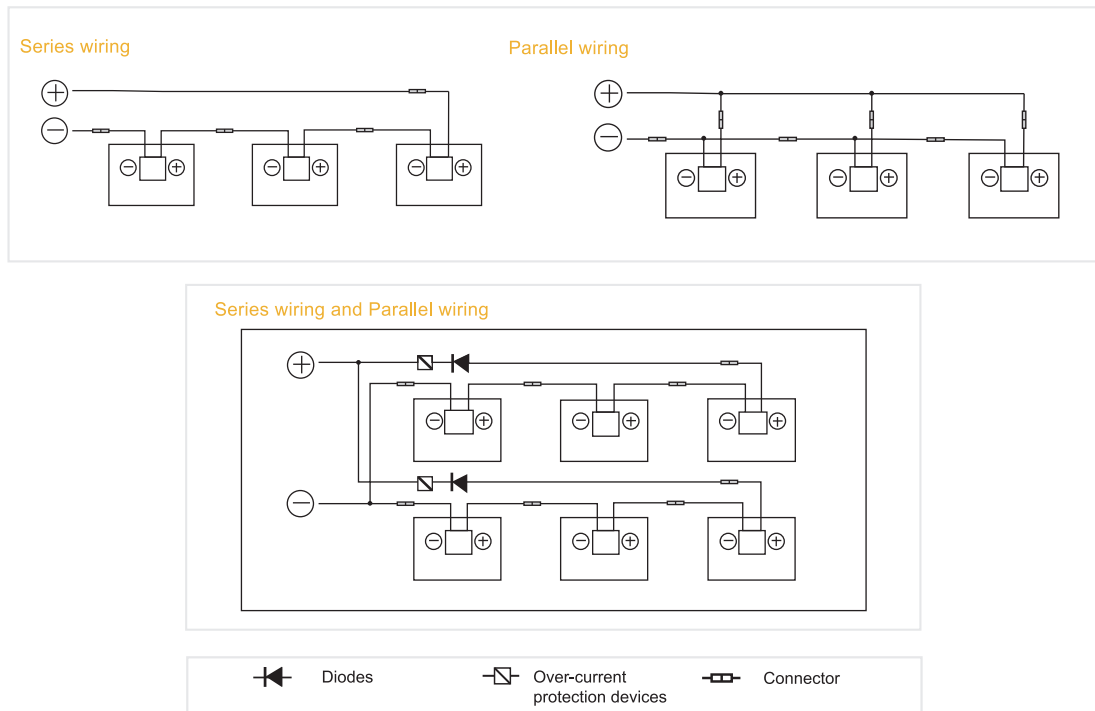
Figure 7: Electrical diagrams of series and parallel wiring
