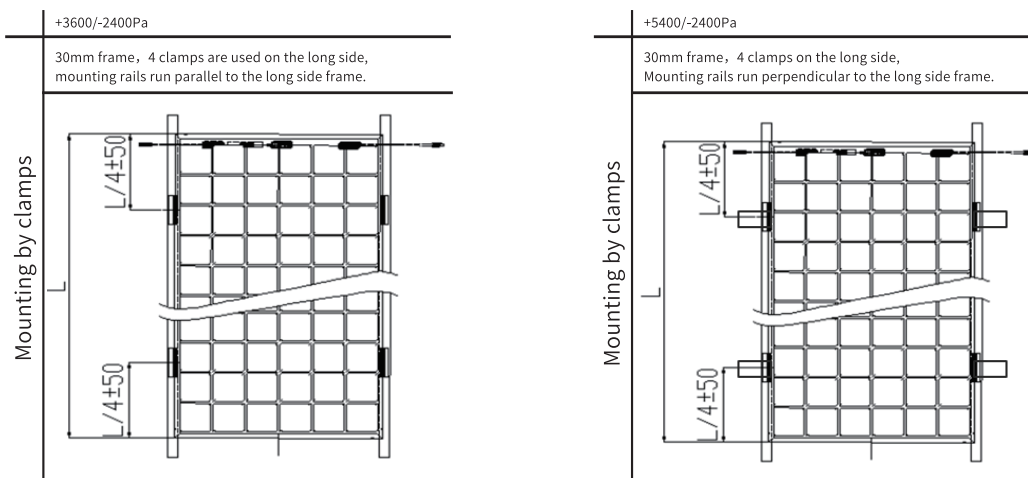
Figure 4 Installation Position and Corresponding Load Relationship (Mounting by clamp)
