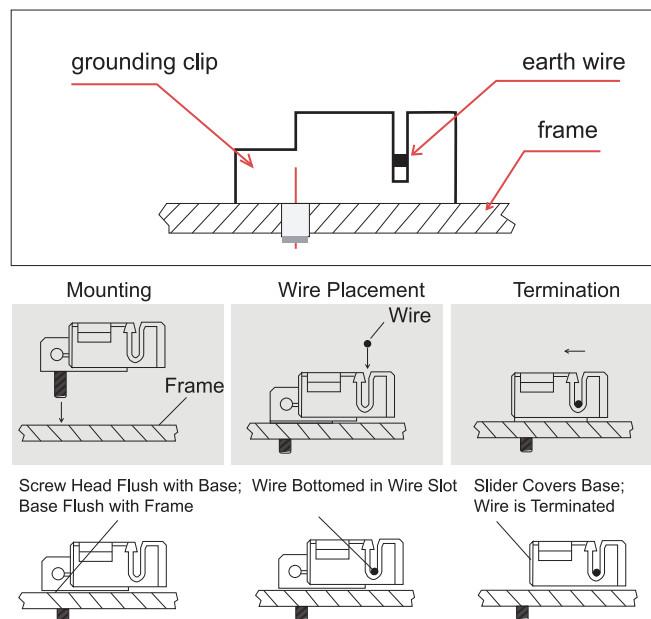
Figure 8: Installation methods
