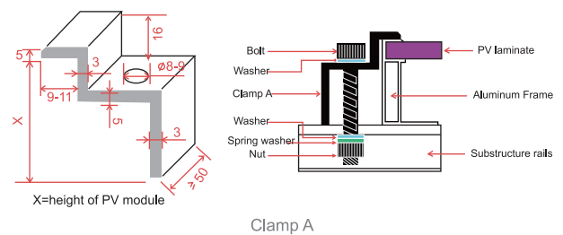
Clamp A
