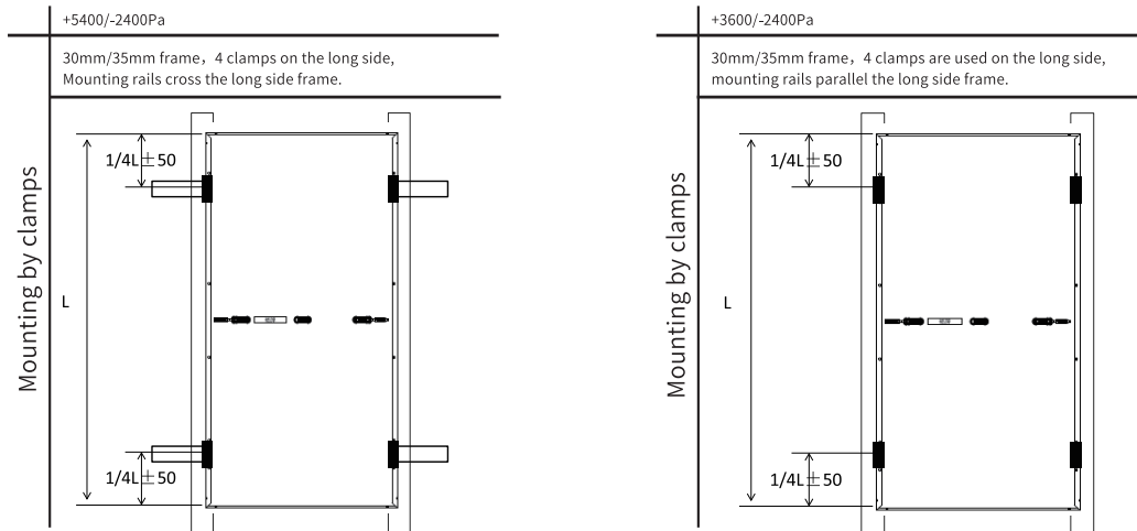
Figure 6 Installation position and corresponding load relation (Mounting by clamp)
