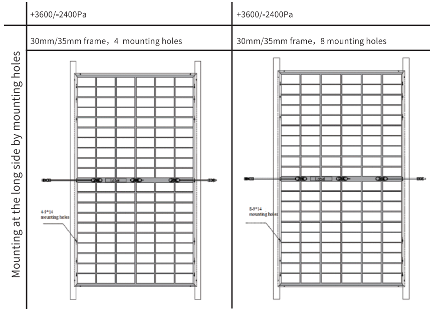
Figure 5 Installation position and corresponding load relation (Mounting by holes)
