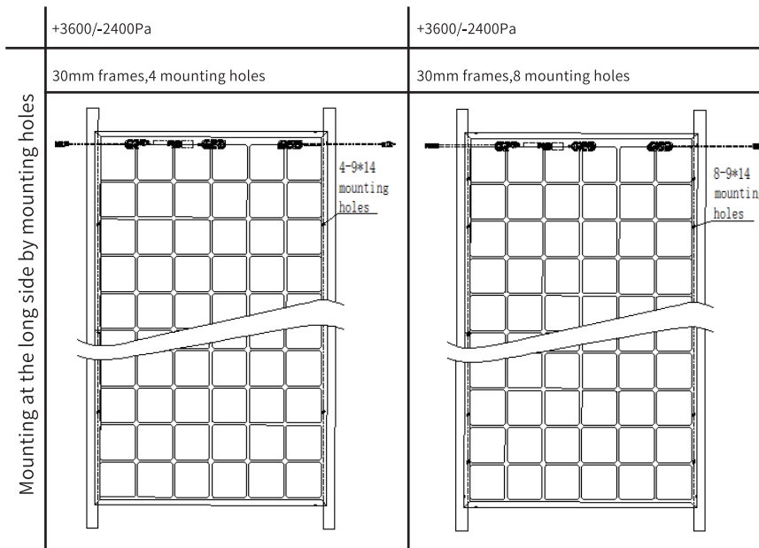
Figure 3 Installation Position and Corresponding Load Relation (Mounting by holes)
