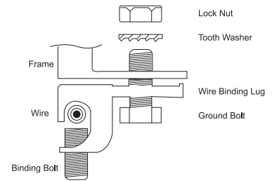
Figure 9: Installation methods
