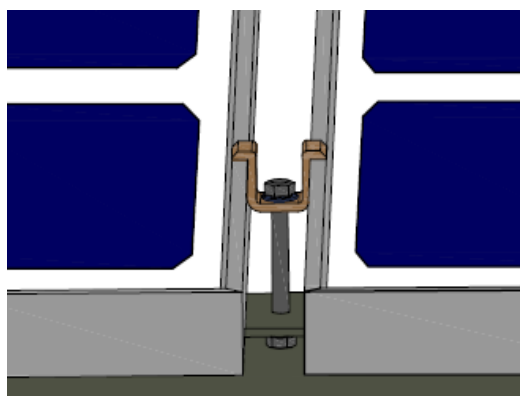
Middle modules installation
