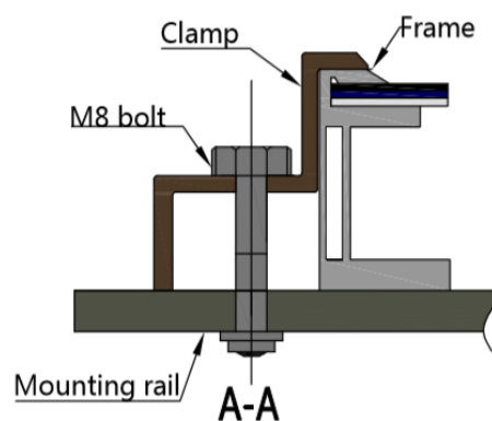
Fringe modules installation
