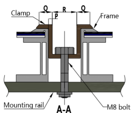
Middle modules installation
