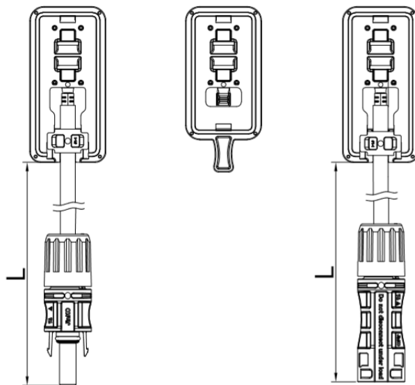
Figure 11 (1): The full module junction box
