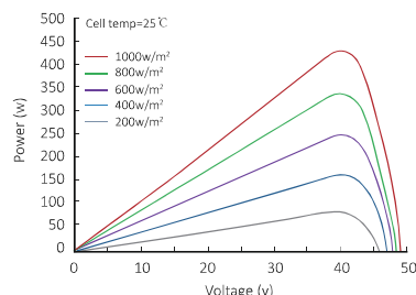
Power-Voltage Curve (LR4-72HIH-440M)
