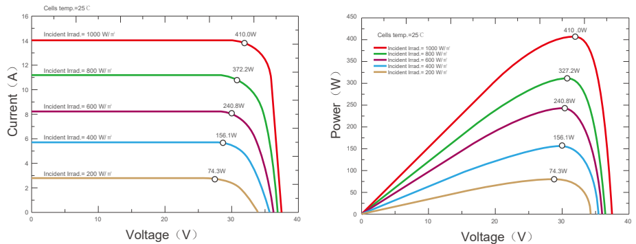
Current-Voltage & Power-Voltage Curves (RMH54-410AB1)
