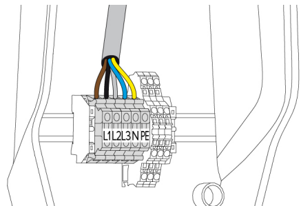
Fig. 7: Power supply connection
