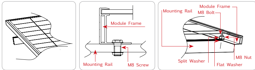
Module installed using Screw Fitting method
