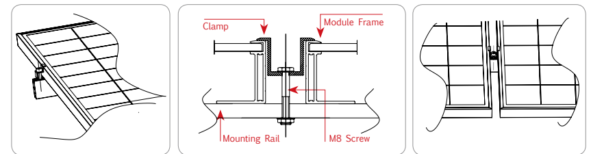
Module installed using Clamp Fitting method
