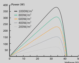
Power-Voltage Curve(380W)
