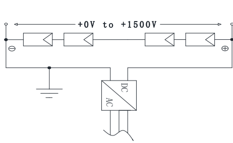
Figure 3. Schematic diagram of grounding potential of inverter
