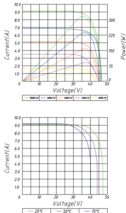
TP672M Pm(W)320
