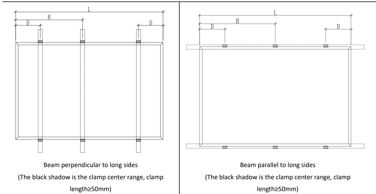
Figure 5 Installation Positions
