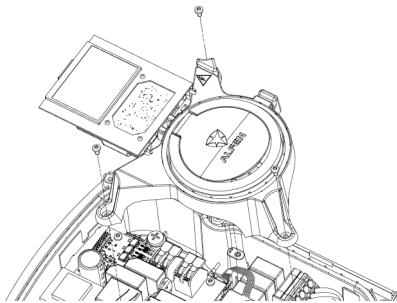
Figure 6: Detach subframe
