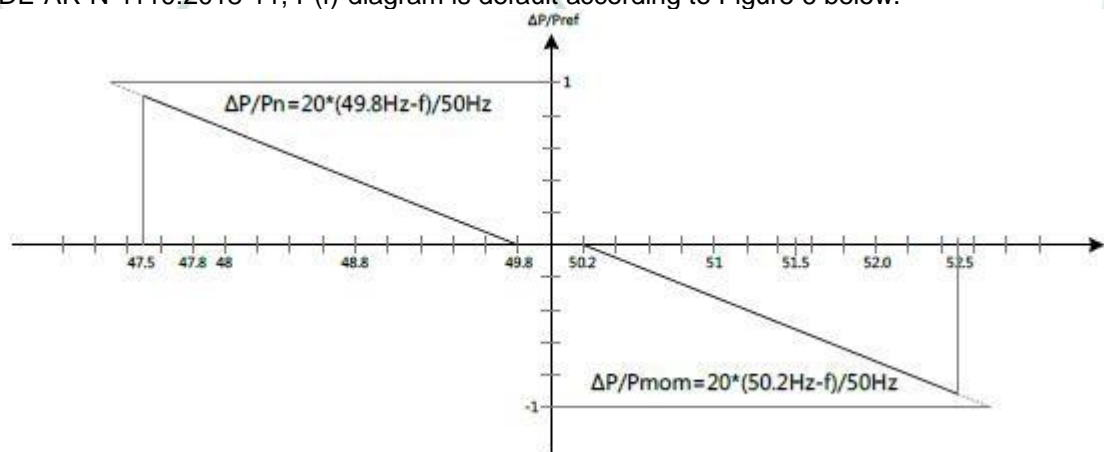
Figure 6 MODEL SOFAR 80KTLX-G3 PV P(f)-diagram
