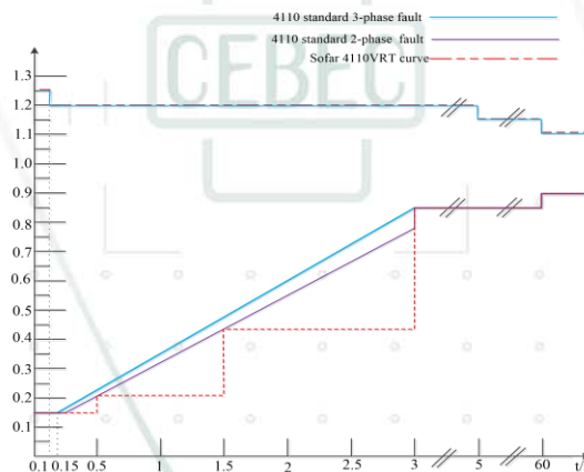
Figure 5 FRT limit curve for SOFAR 80KTLX-G3 PV
