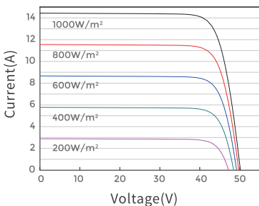
Current-Voltage Curve JAM72D30-575/LB
