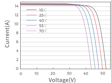
Current-Voltage Curve JAM72D30-575/LB
