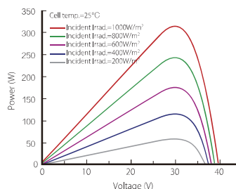
Power-Voltage Curve (LR6-60PH-310M)
