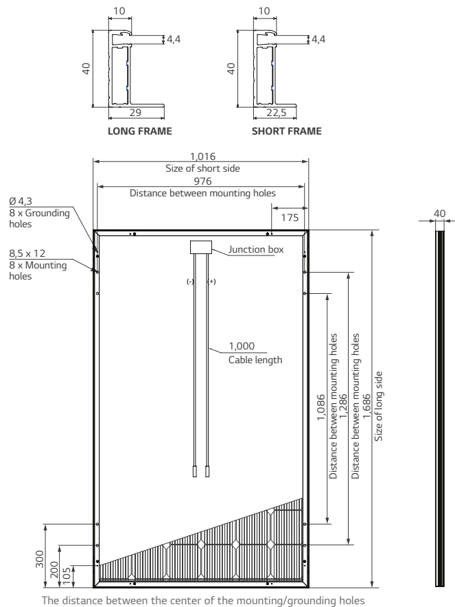
The distance between the center of the mounting/grounding holes
