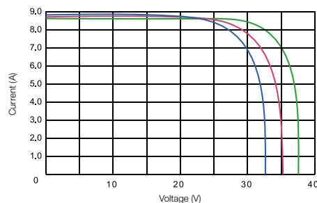
TP660P Pm(W)240
