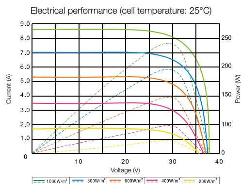
TP660P Pm(W)240
